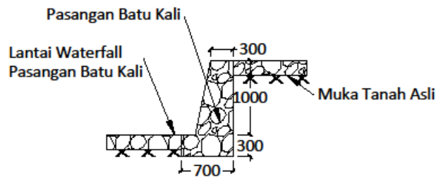
DETAIL 1 SKALA NTS
