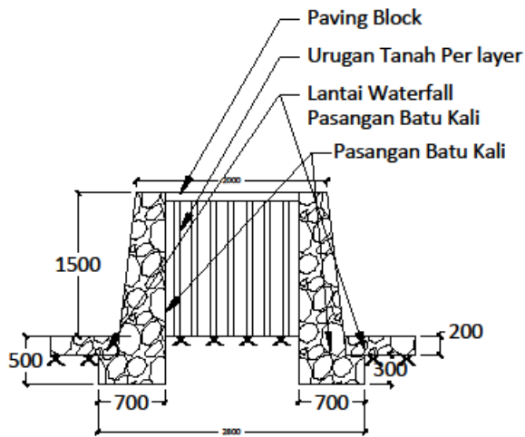
DETAIL 2 SKALA NTS
