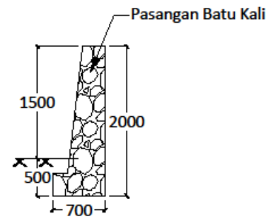
DETAIL 3 SKALA NTS
