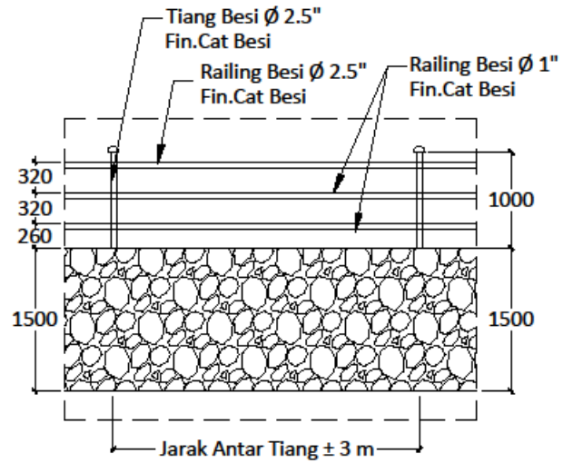
DETAIL HAND RAILING SKALA NTS
